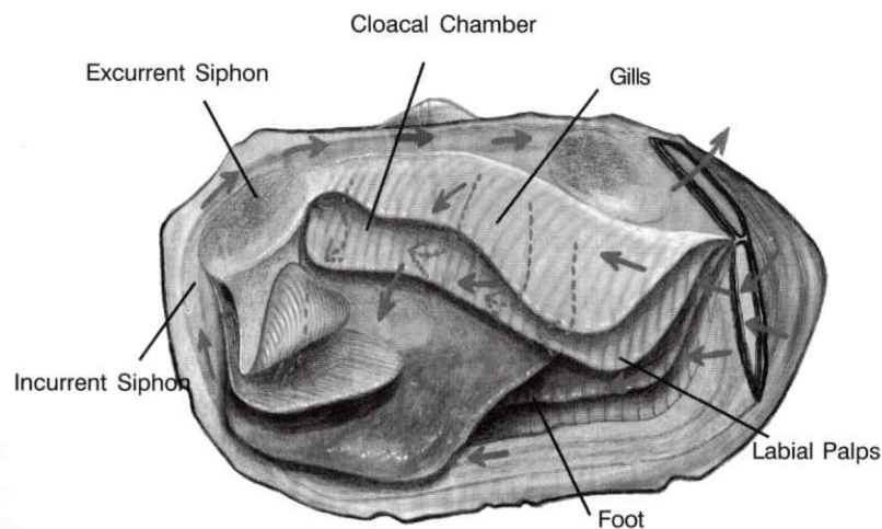
Figure 3: Water circulation and food particle flow. Solid lines illustrate water flow while dotted lines track trapped food particles and their flow into the mouth.
