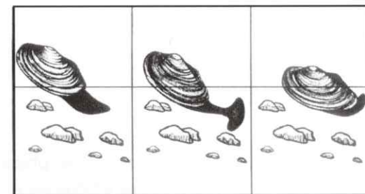
Figure 6: Foot extension, expansion, and contraction demonstrating clam movement.
