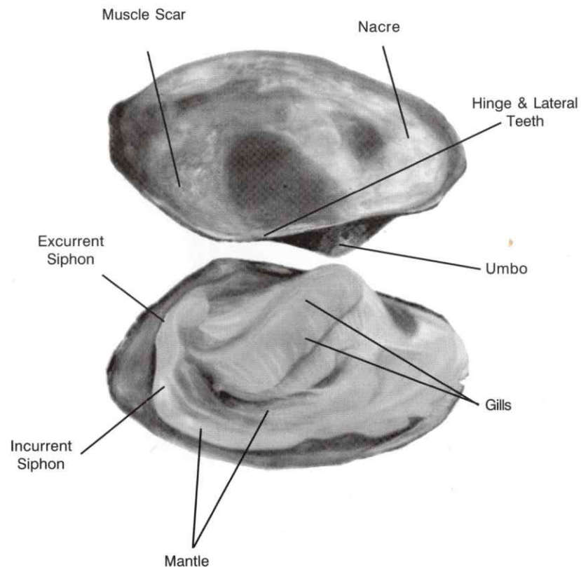
Figure 2: Internal view with mantle in place.
